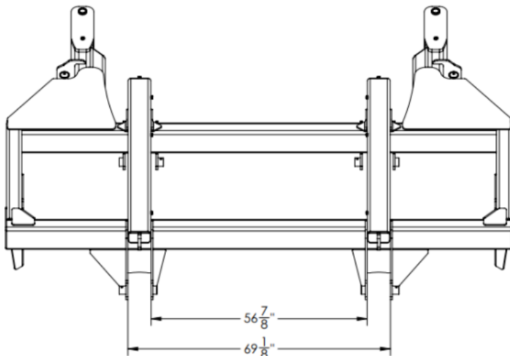
Detail D
