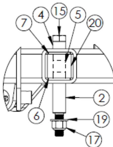
DETAIL D SCALE 1 : 8
