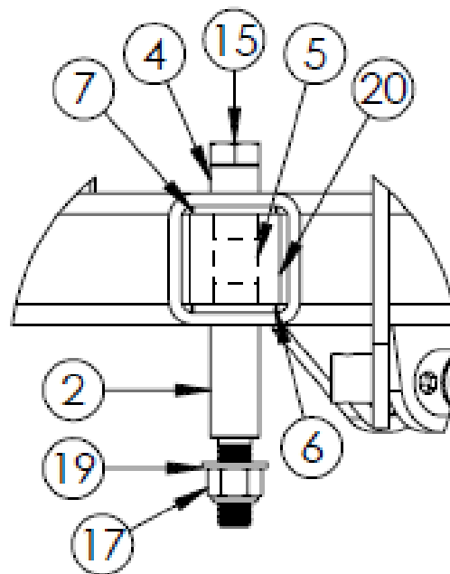
DETAIL D SCALE 1 : 8
