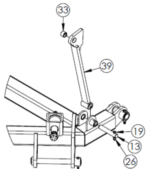
DETAIL G SCALE 1 : 14
