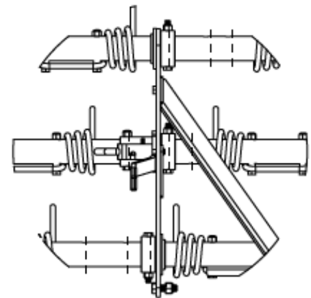
DETAIL C SCALE 1 : 14
