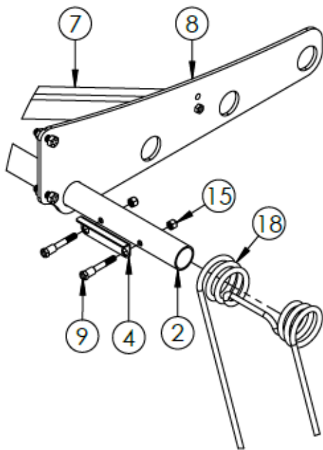
DETAIL A SCALE 1 : 12
