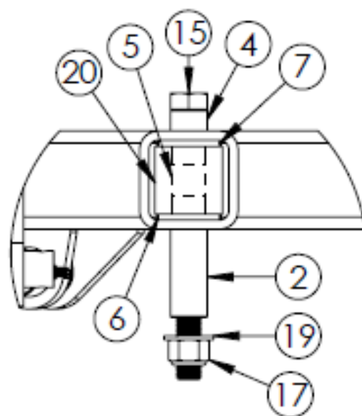
DETAIL D SCALE 1 : 8
