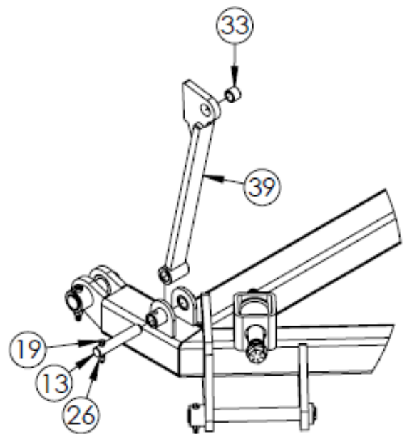
DETAIL G SCALE 1 : 15
