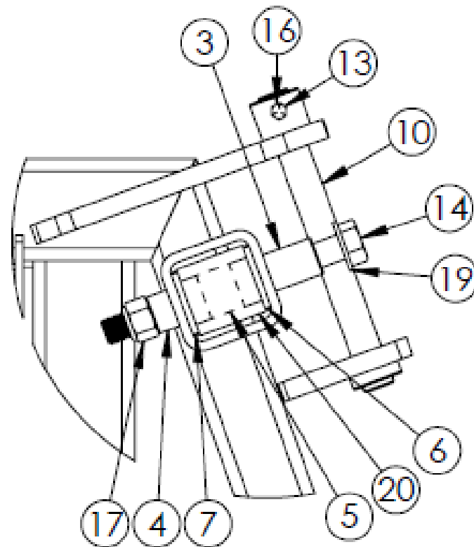
DETAIL A SCALE 1 : 8
