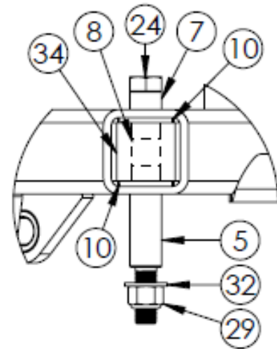
DETAIL E SCALE 1 : 8
