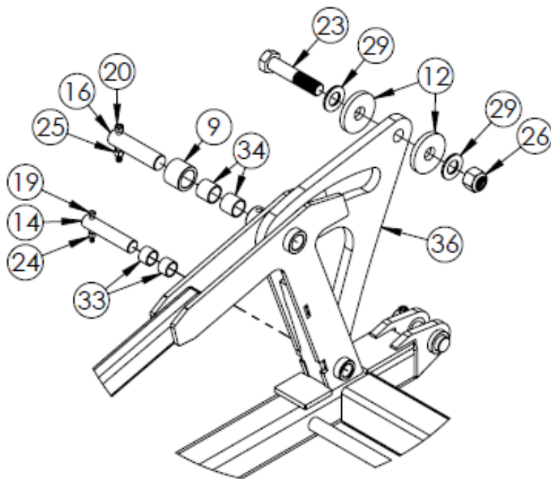
DETAIL F SCALE 1 : 14
