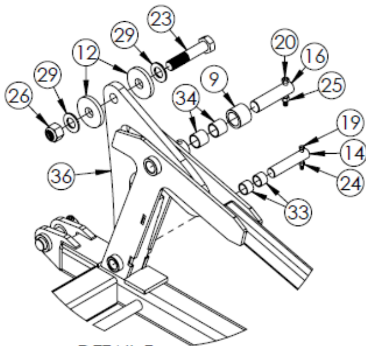
DETAIL F SCALE 1 : 14
