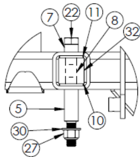
DETAIL E SCALE 1 : 8
