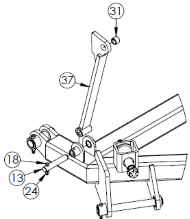
DETAIL B SCALE 2 : 25
