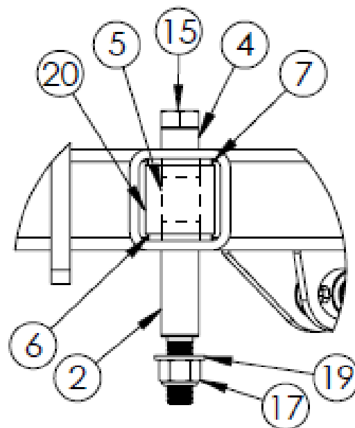
DETAIL D SCALE 1 : 8
