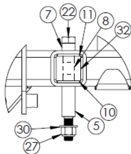
DETAIL E SCALE 1 : 8
