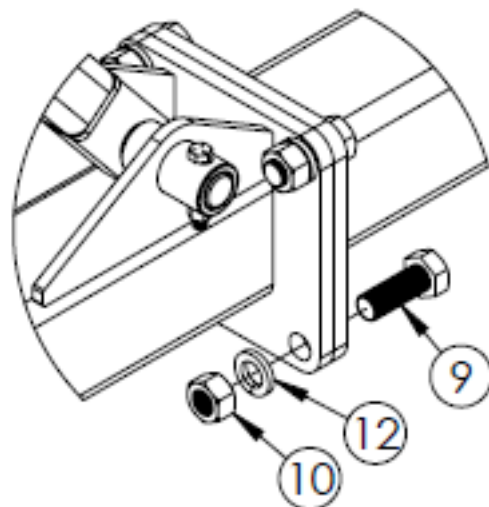
DETAIL A SCALE 1 : 7
