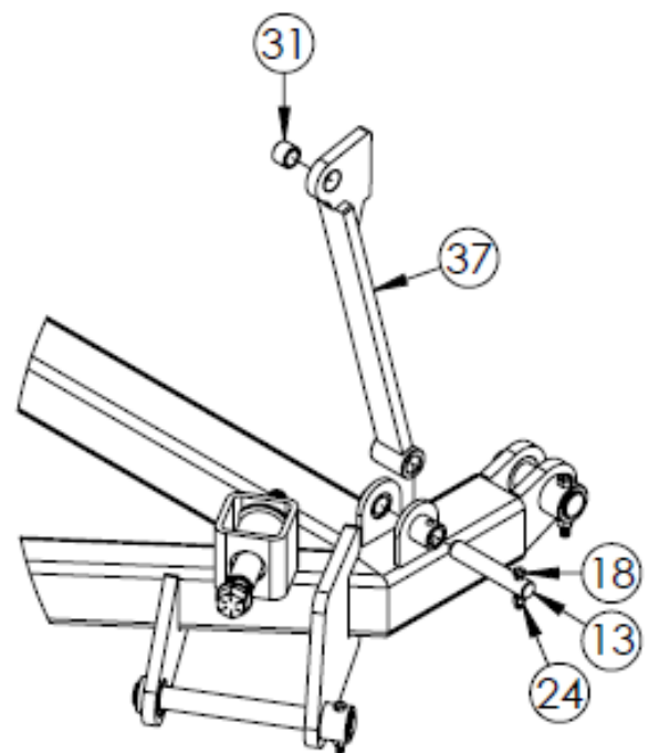
DETAIL G SCALE 1 : 14
