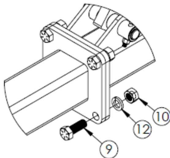
DETAIL A SCALE 1 : 7
