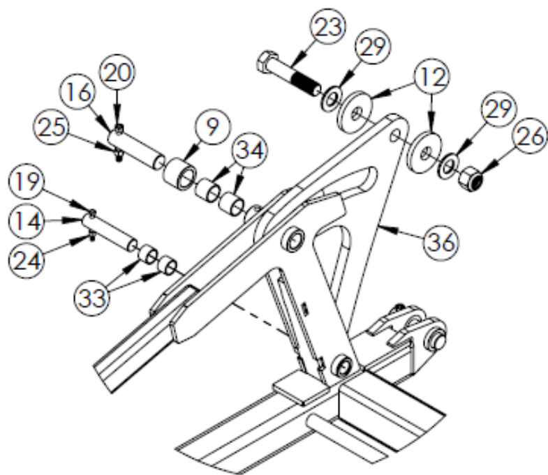
DETAIL F SCALE 1 : 14
