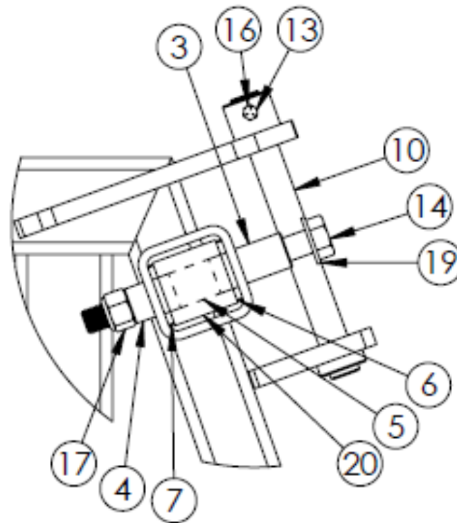
DETAIL A SCALE 1 : 8
