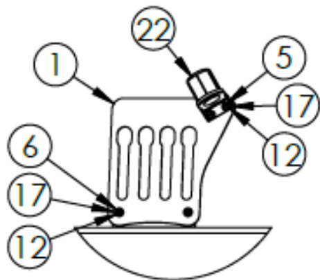
DETAIL C SCALE 1 : 15
