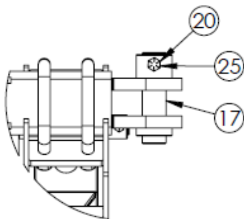
DETAIL A SCALE 1 : 8
