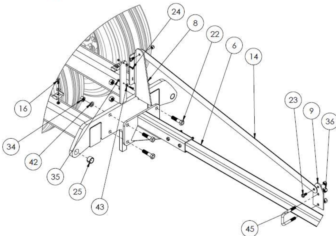
DETAIL G SCALE 1 : 10
