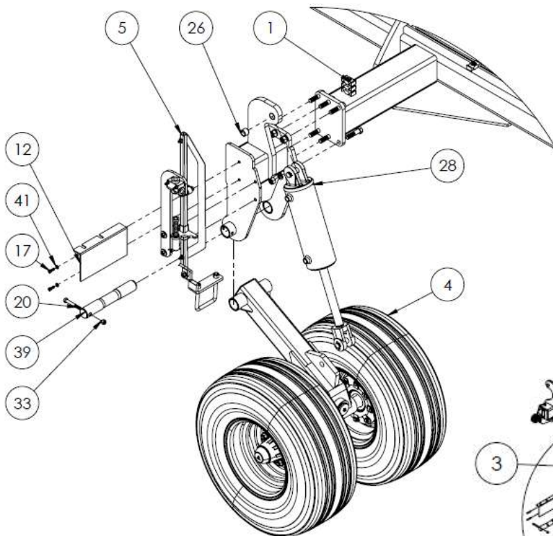
DETAIL A SCALE 1 : 15
