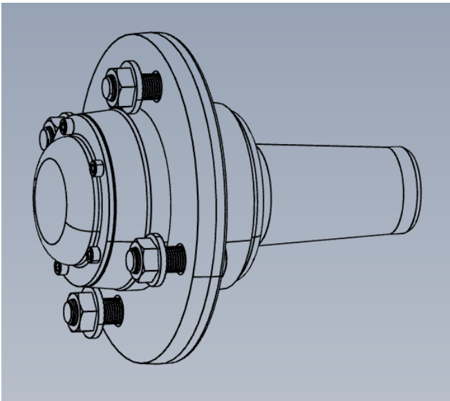
R9903020- Tapered Spindle. Maintenance Free. Service Kit not available.
