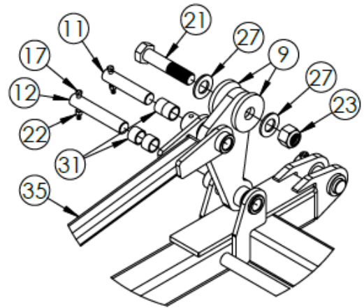
DETAIL F SCALE 1 : 12
