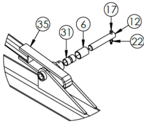
DETAIL G SCALE 1 : 12
